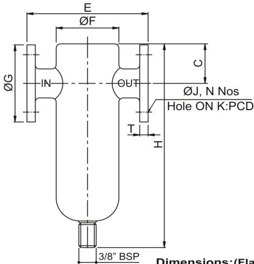
Dimensions:(Flanged As Per 'D' Table)(Only Thickness as per Table F) (All Dimensions are in mm)
